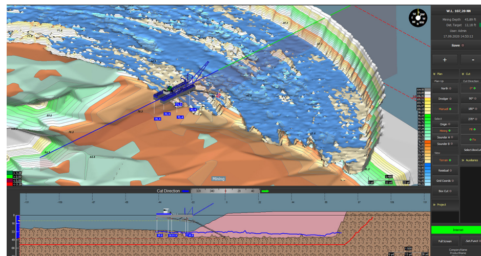
FIGURE 2 Operator's view of a touchscreen monitor installed on a cutter-suction dredge.
