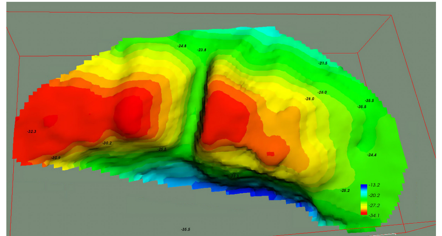
FIGURE 7 Plan view of reservoir dredging project.
