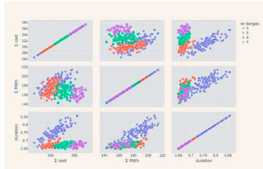
FIGURE 5 Scatter plot of all KPIs vs all KPIs for every per scenario. The scenarios with two and three barges have been left out to be able to focus on the data range for the most likely candidates with four or more barges.
