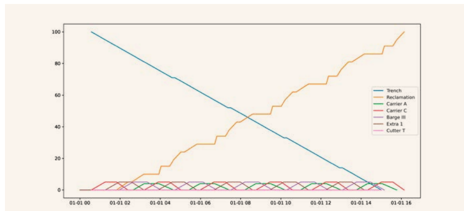
FIGURE 2 The cumulative amount of material per vessel or site in a random example case.
