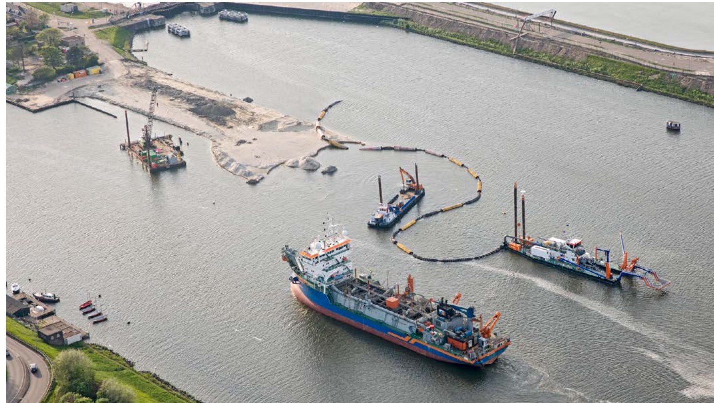
FIGURE 9 Cutter suction dredger Biesbosch, trailing hopper suction dredger HAM 317 and auxiliary equipment working on the new sea lock in IJmuiden, the Netherlands. 30% of the Biesbosch's standard fuel was diluted with a biofuel component, a safe mix ratio that does not damage the engine.
