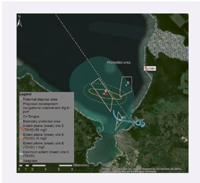
FIGURE 11 Extent plume disposal site E using TSHD.
