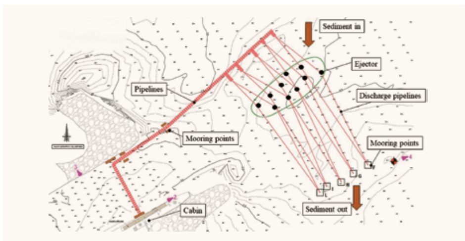
FIGURE 2 Location of ejectors in the Cervia plant.
